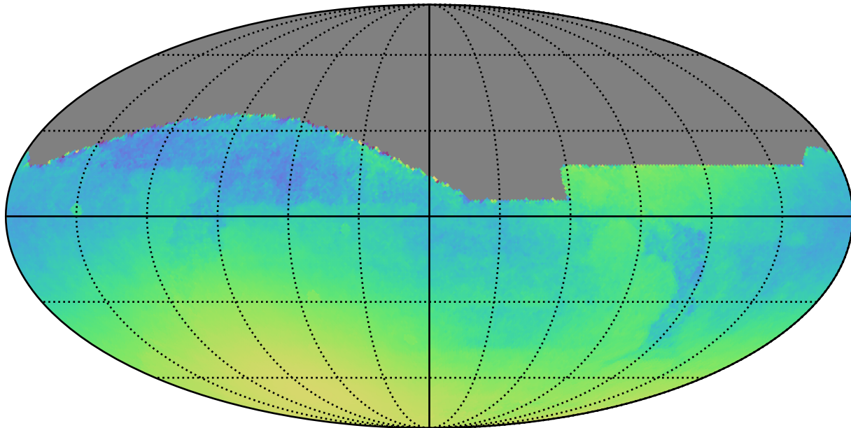
extra_ss_neo3_v3.4_10yrs : Normalized Parallax Uncert @ 22.4
