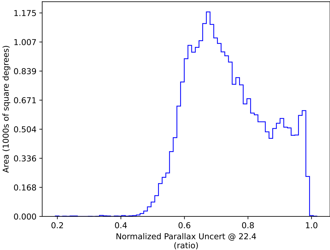
extra_ss_neo3_v3.4_10yrs : Normalized Parallax Uncert @ 22.4
