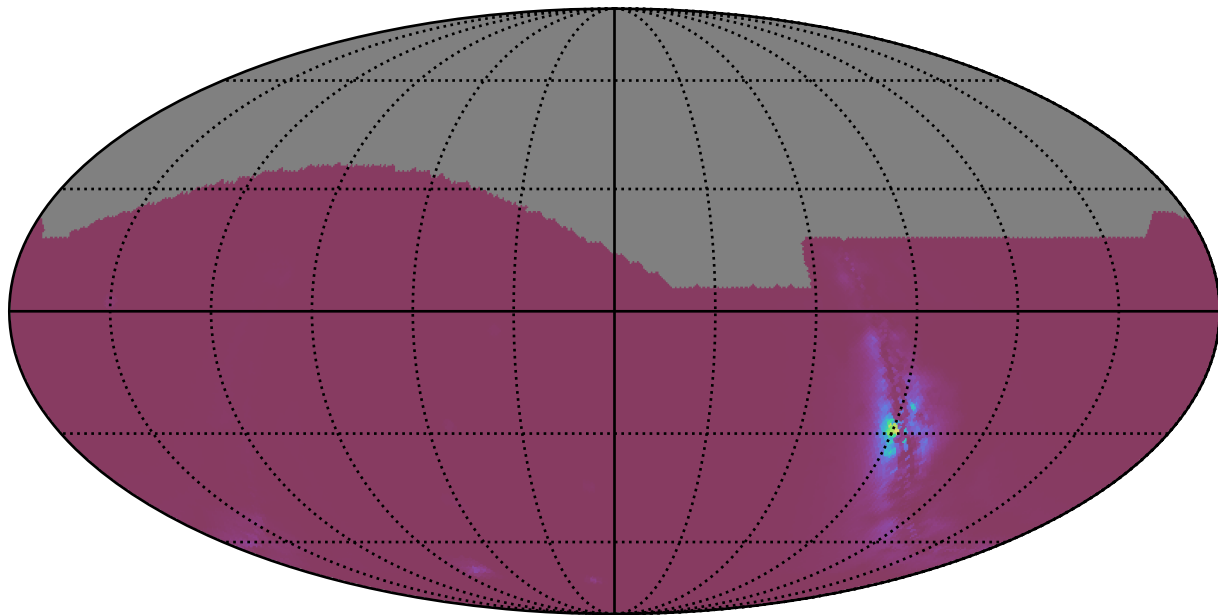
extra_ss_neo3_v3.4_10yrs : NlcPoints
