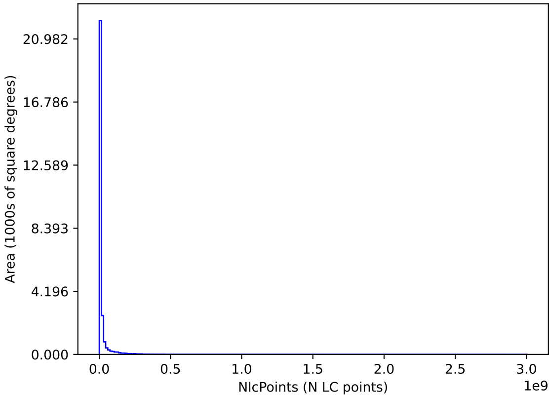
extra_ss_neo3_v3.4_10yrs : NlcPoints
