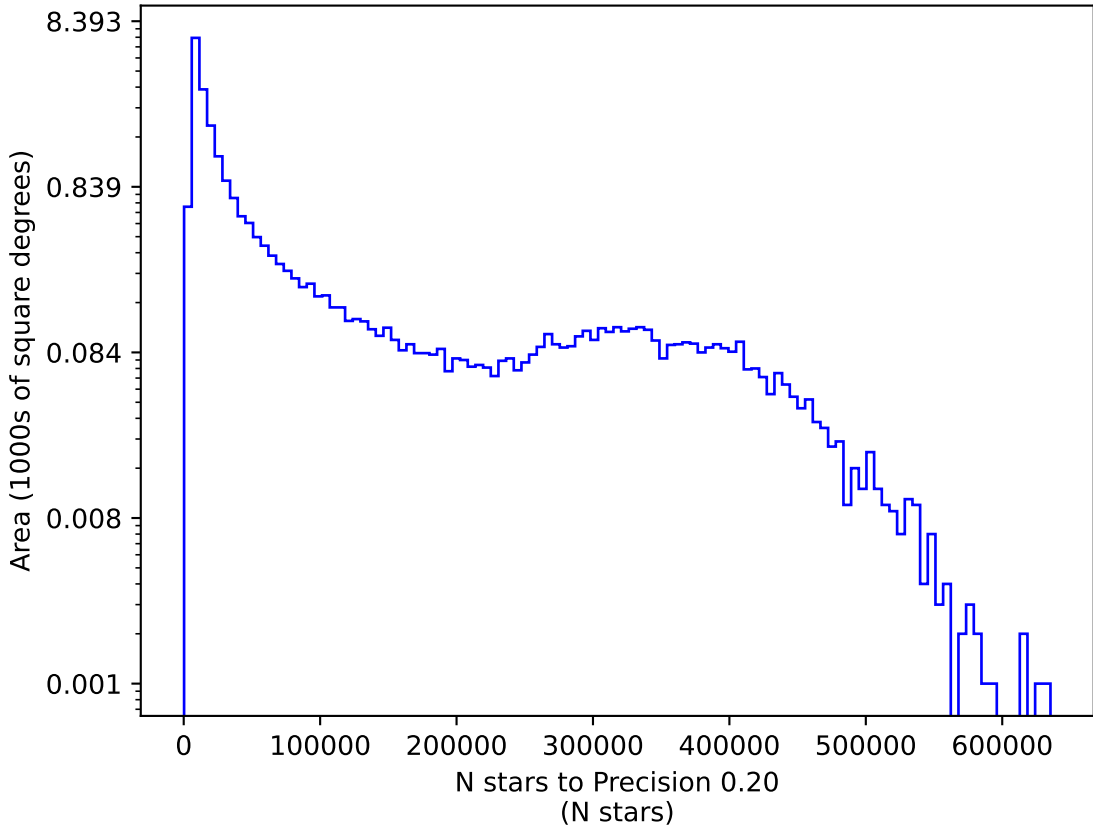
extra_ss_neo3_v3.4_10yrs y: N stars to Precision 0.20
