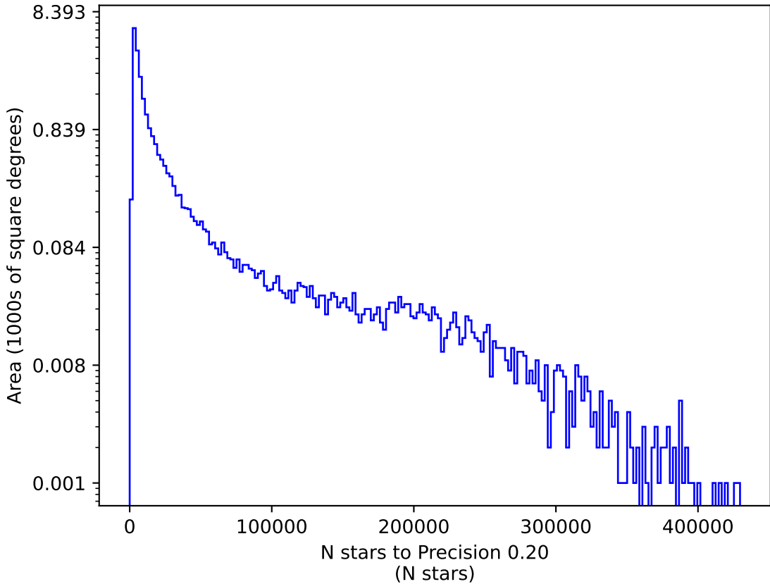
extra_ss_neo3_v3.4_10yrs u: N stars to Precision 0.20
