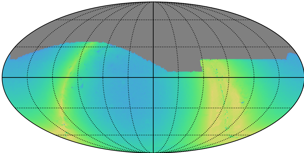
extra_ss_neo3_v3.4_10yrs r: N stars to Precision 0.20
