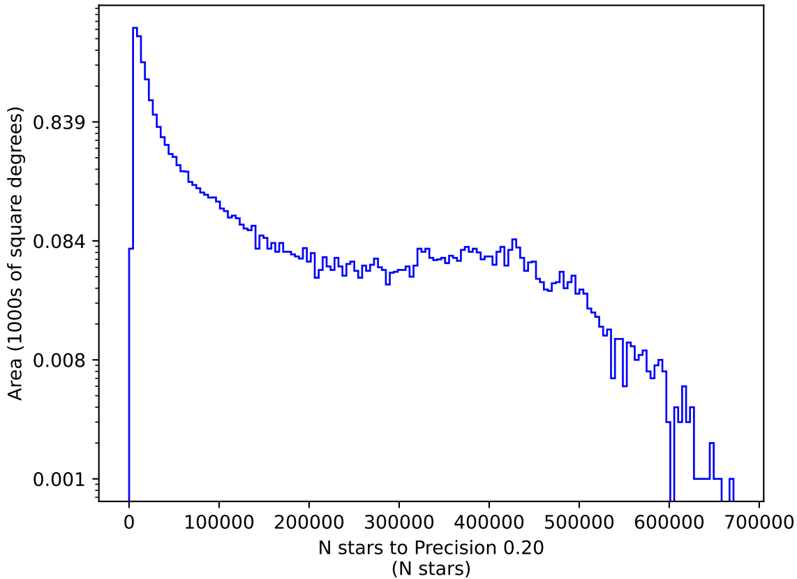
extra_ss_neo3_v3.4_10yrs r: N stars to Precision 0.20
