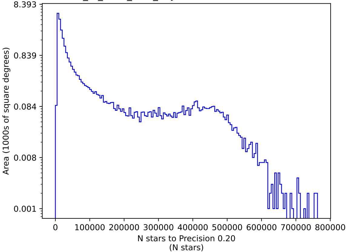
extra_ss_neo3_v3.4_10yrs i: N stars to Precision 0.20
