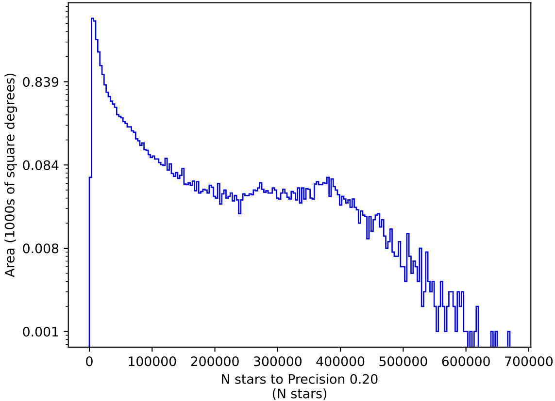
extra_ss_neo3_v3.4_10yrs g: N stars to Precision 0.20
