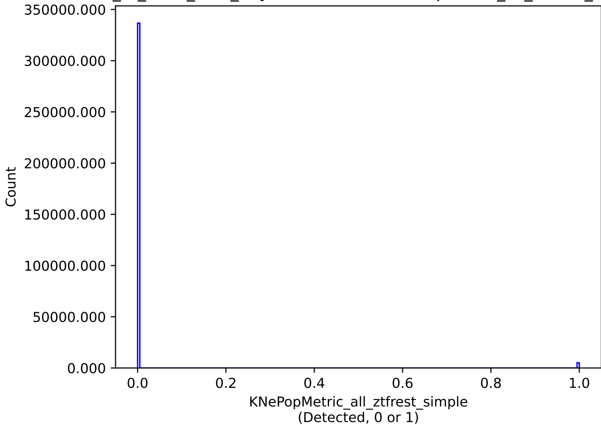
extra_ss_neo3_v3.4_10yrs all models: KNePopMetric_all_ztfrest_simple
