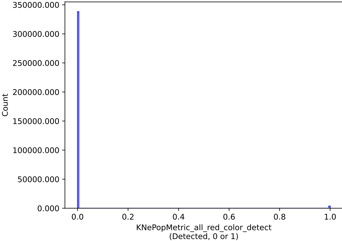
extra_ss_neo3_v3.4_10yrs all models: KNePopMetric_all_red_color_detect
