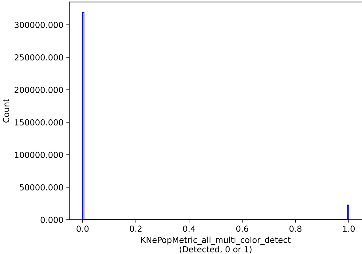
extra_ss_neo3_v3.4_10yrs all models: KNePopMetric_all_multi_color_detect
