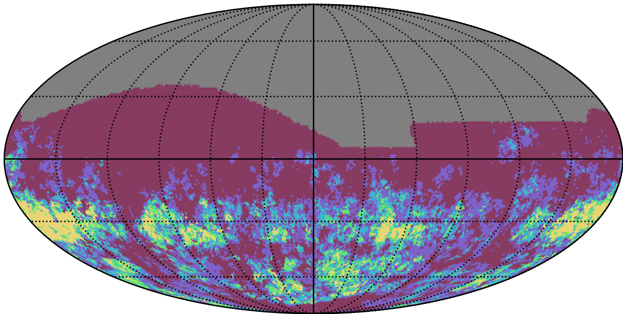
extra_ss_neo3_v3.4_10yrs r band: Gaps_7hr
