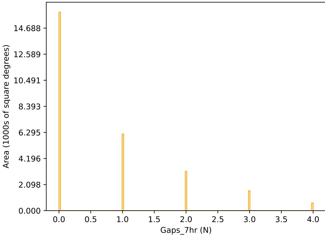
extra_ss_neo3_v3.4_10yrs r band: Gaps_7hr
