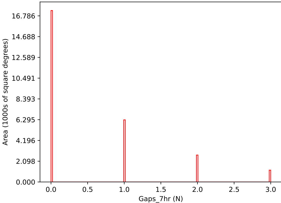
extra_ss_neo3_v3.4_10yrs i band: Gaps_7hr
