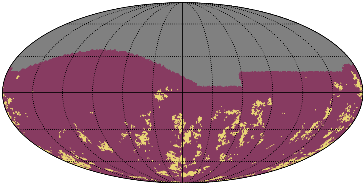
extra_ss_neo3_v3.4_10yrs g band: Gaps_7hr
