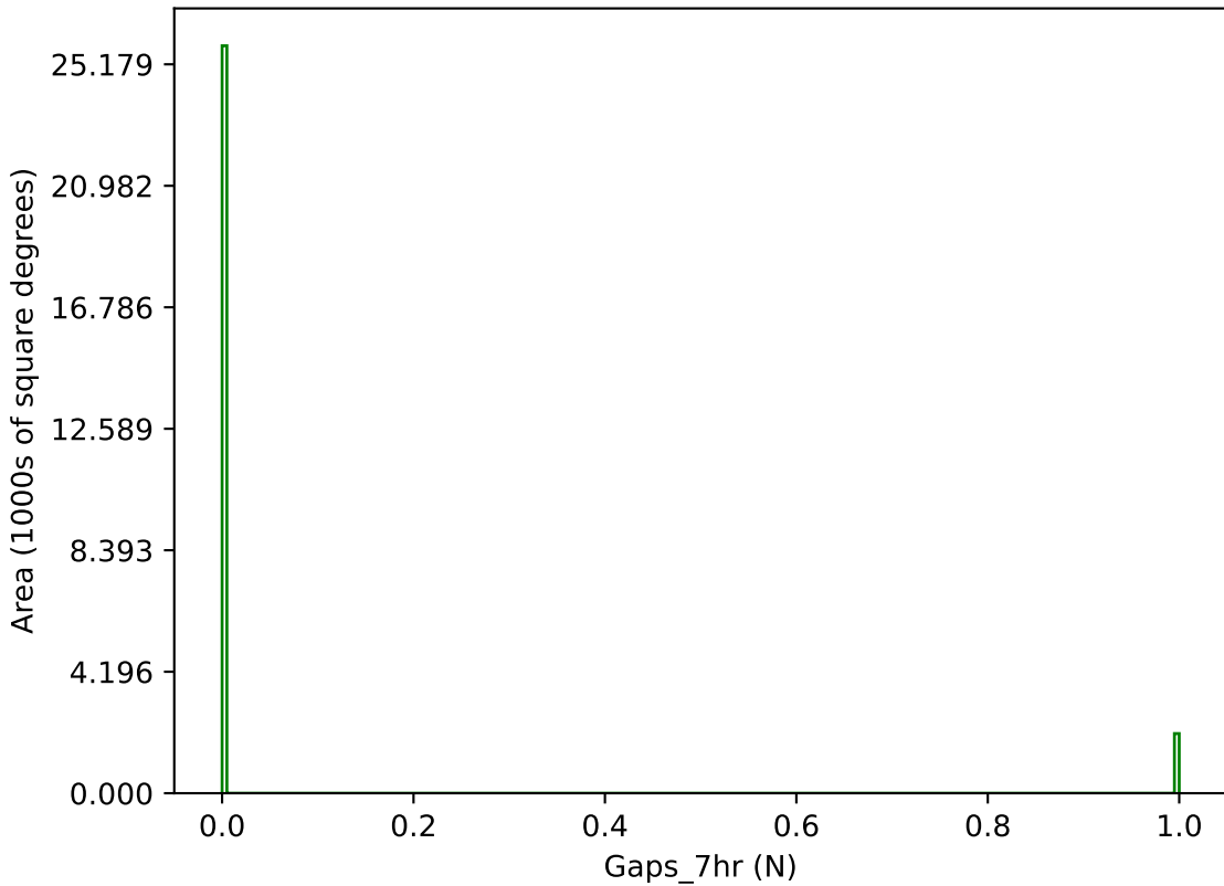
extra_ss_neo3_v3.4_10yrs g band: Gaps_7hr
