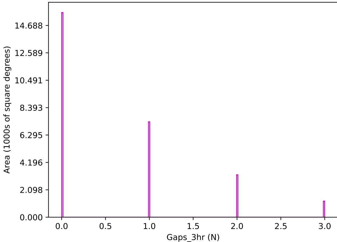
extra_ss_neo3_v3.4_10yrs z band: Gaps_3hr
