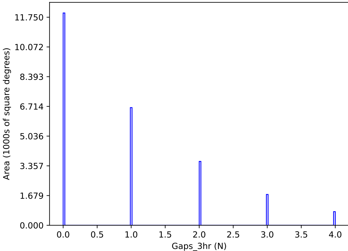
extra_ss_neo3_v3.4_10yrs y band: Gaps_3hr
