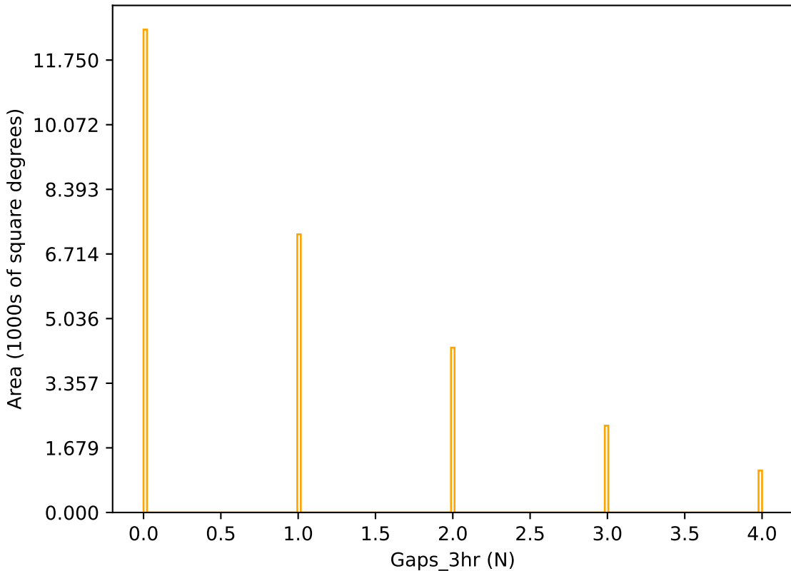
extra_ss_neo3_v3.4_10yrs r band: Gaps_3hr
