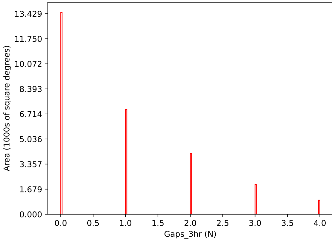
extra_ss_neo3_v3.4_10yrs i band: Gaps_3hr
