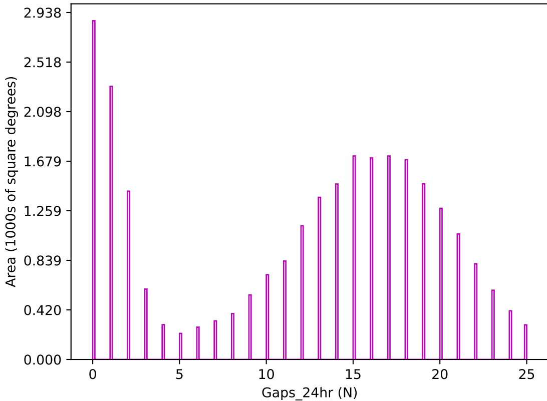
extra_ss_neo3_v3.4_10yrs z band: Gaps_24hr
