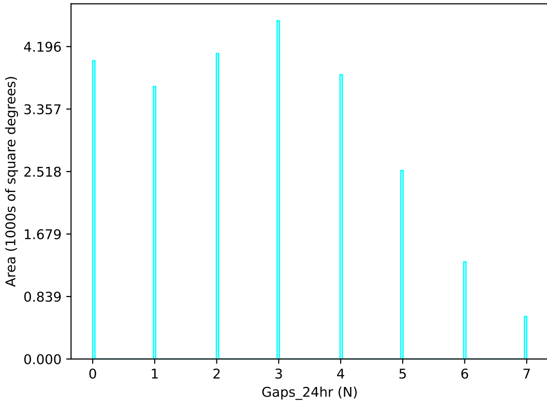
extra_ss_neo3_v3.4_10yrs u band: Gaps_24hr
