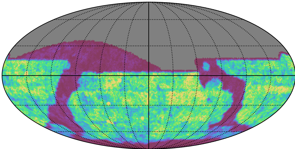
extra_ss_neo3_v3.4_10yrs r band: Gaps_24hr
