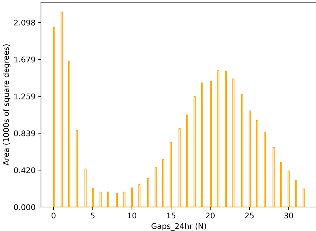
extra_ss_neo3_v3.4_10yrs r band: Gaps_24hr
