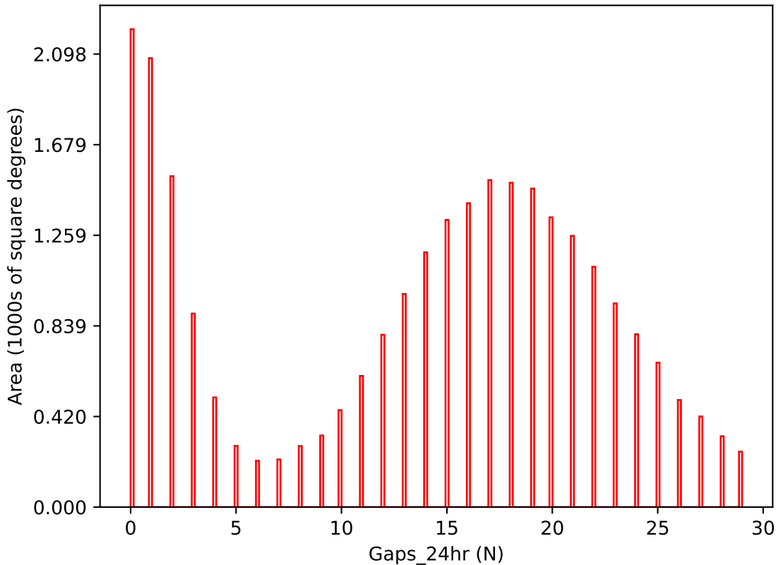
extra_ss_neo3_v3.4_10yrs i band: Gaps_24hr
