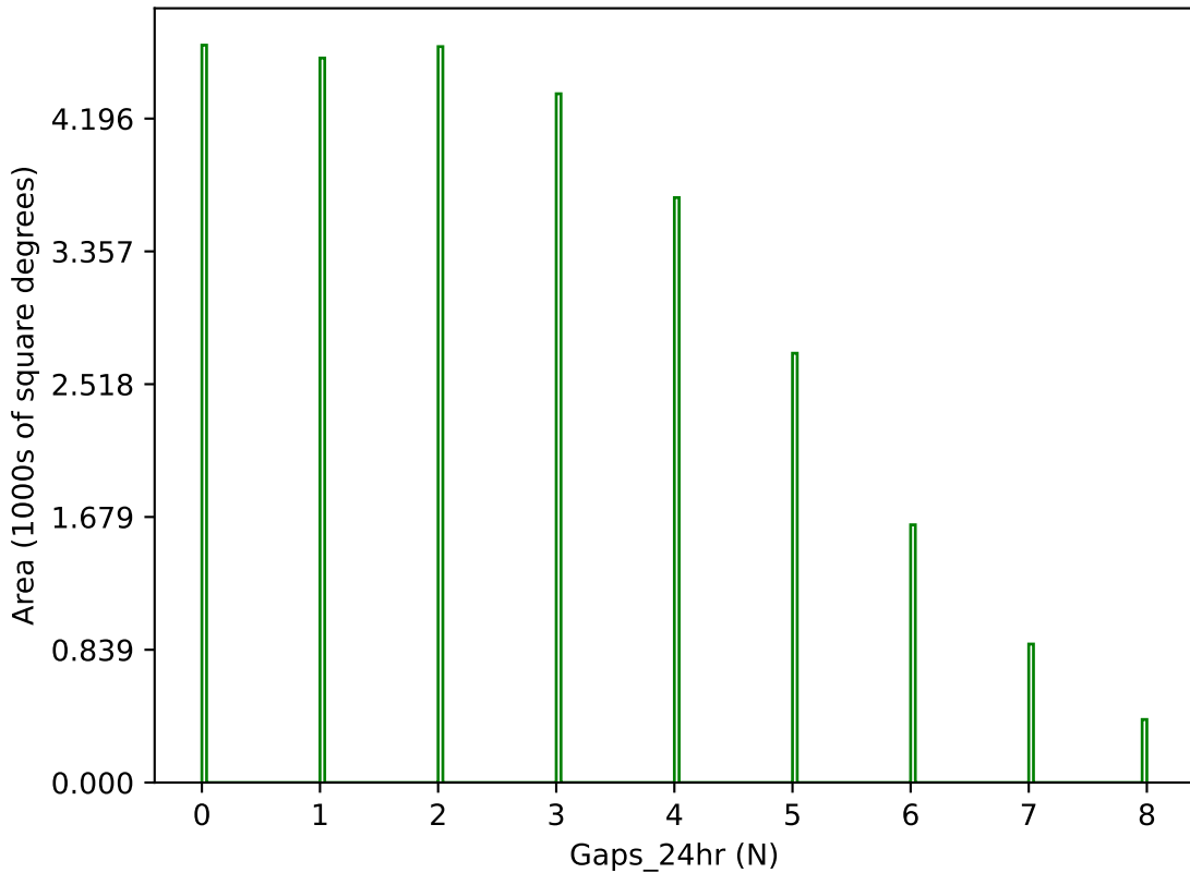
extra_ss_neo3_v3.4_10yrs g band: Gaps_24hr
