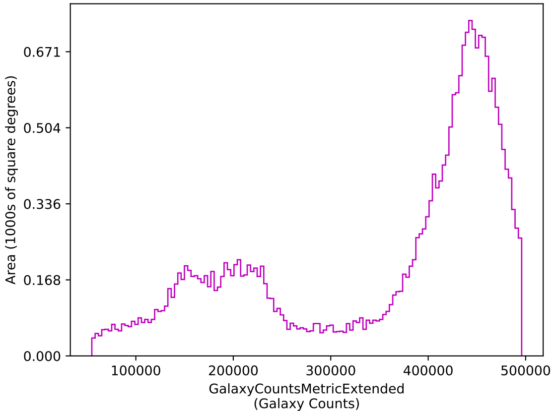
extra_ss_neo3_v3.4_10yrs z: GalaxyCountsMetricExtended
