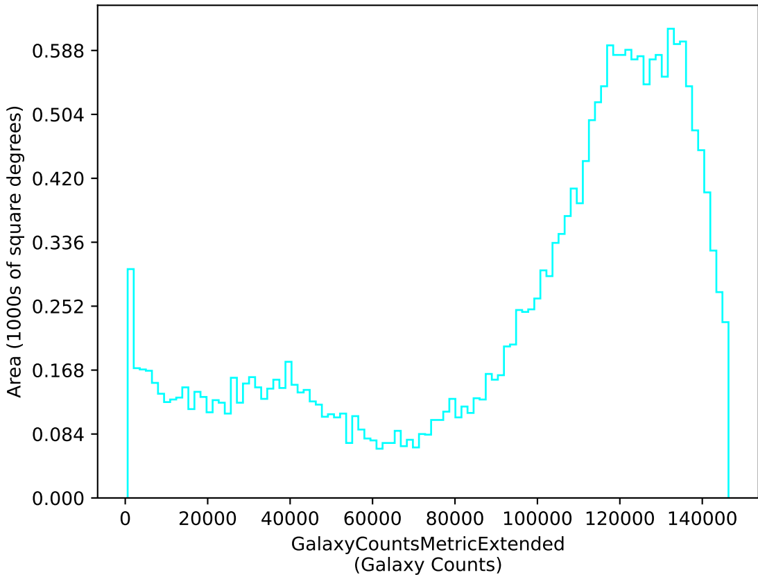
extra_ss_neo3_v3.4_10yrs u: GalaxyCountsMetricExtended
