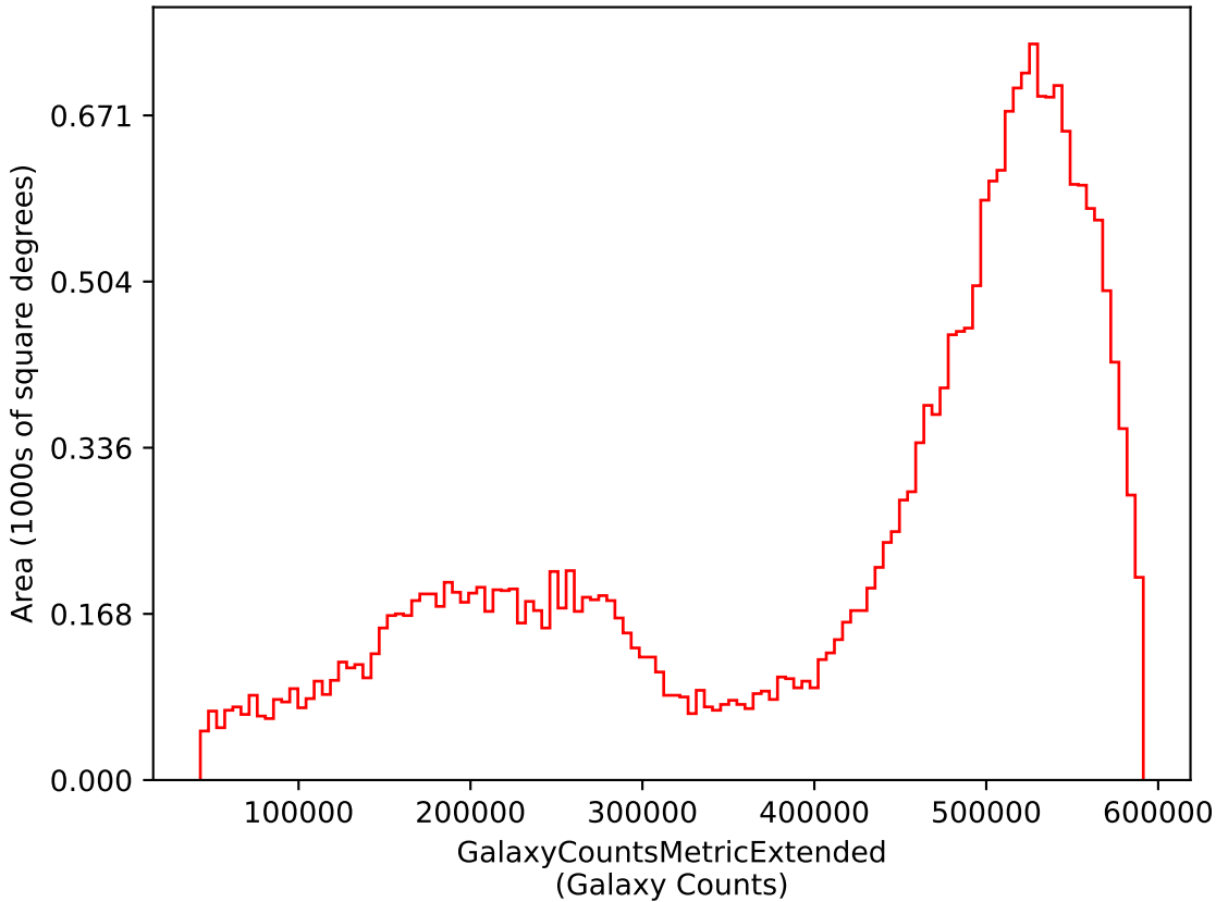
extra_ss_neo3_v3.4_10yrs i: GalaxyCountsMetricExtended
