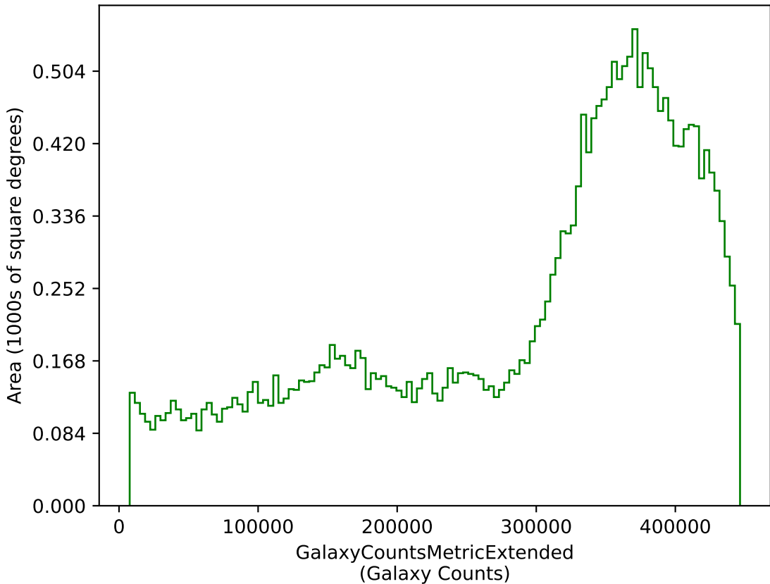
extra_ss_neo3_v3.4_10yrs g: GalaxyCountsMetricExtended
