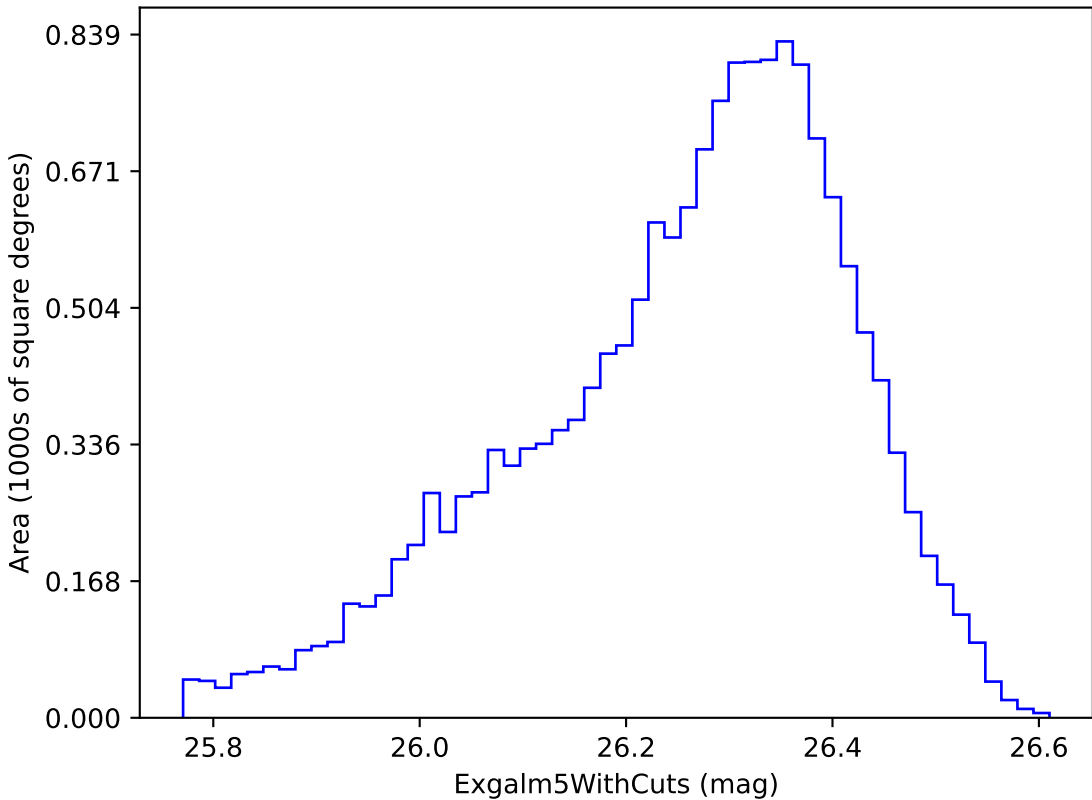
extra_ss_neo3_v3.4_10yrs i band non-DD year 8: ExgalM5WithCuts
