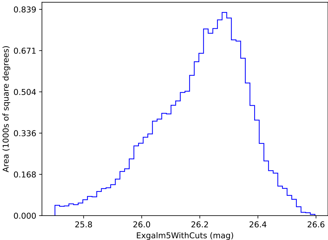
extra_ss_neo3_v3.4_10yrs i band non-DD year 7: Exgalml5WithCuts
