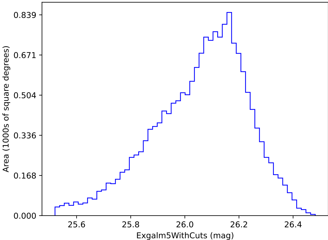
extra_ss_neo3_v3.4_10yrs i band non-DD year 5: ExgalM5WithCuts
