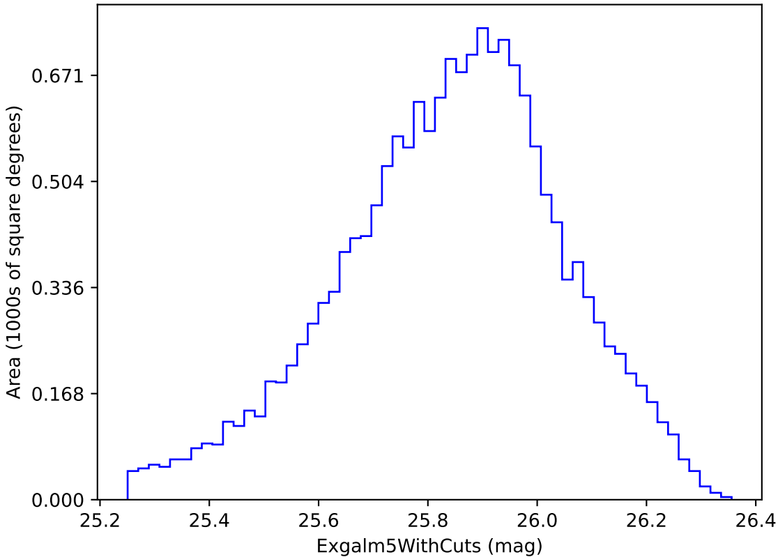
extra_ss_neo3_v3.4_10yrs i band non-DD year 3: ExgalM5WithCuts
