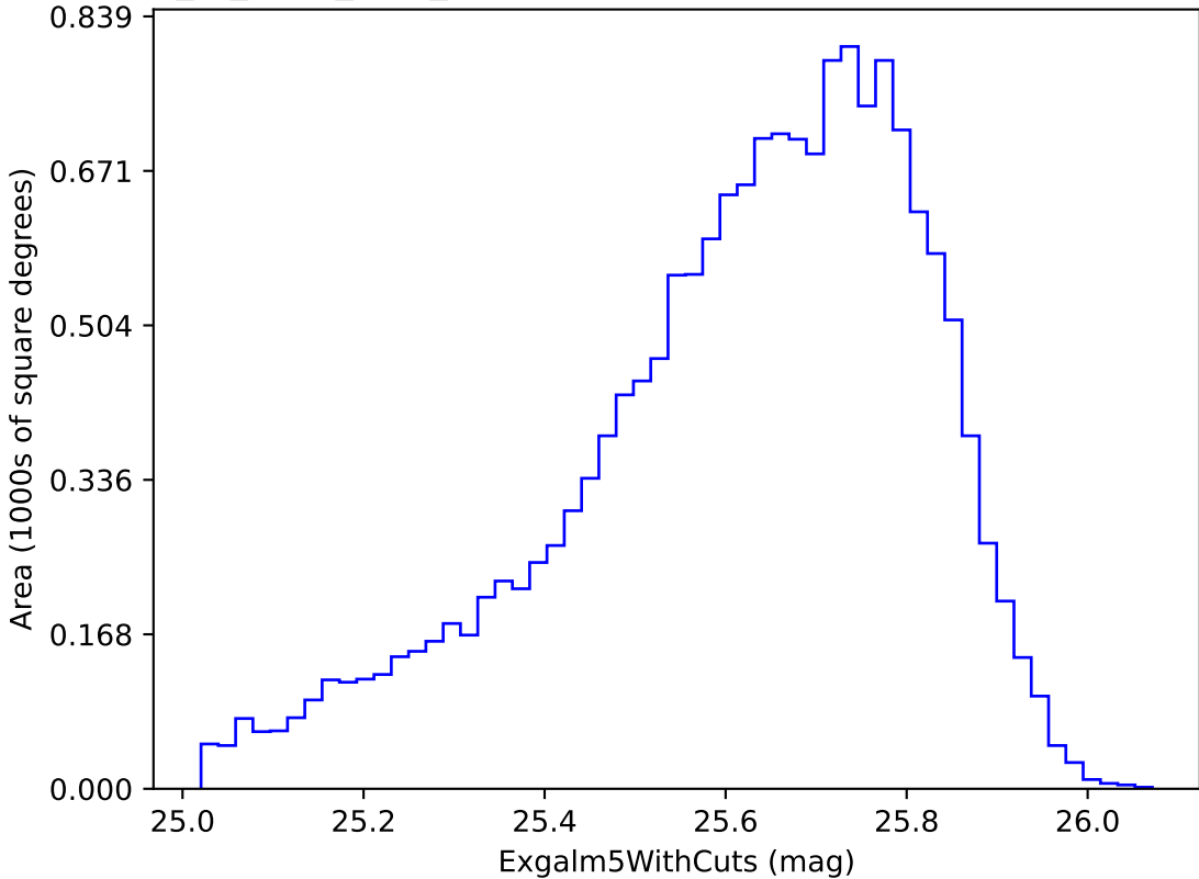
extra_ss_neo3_v3.4_10yrs i band non-DD year 2: ExgalM5WithCuts
