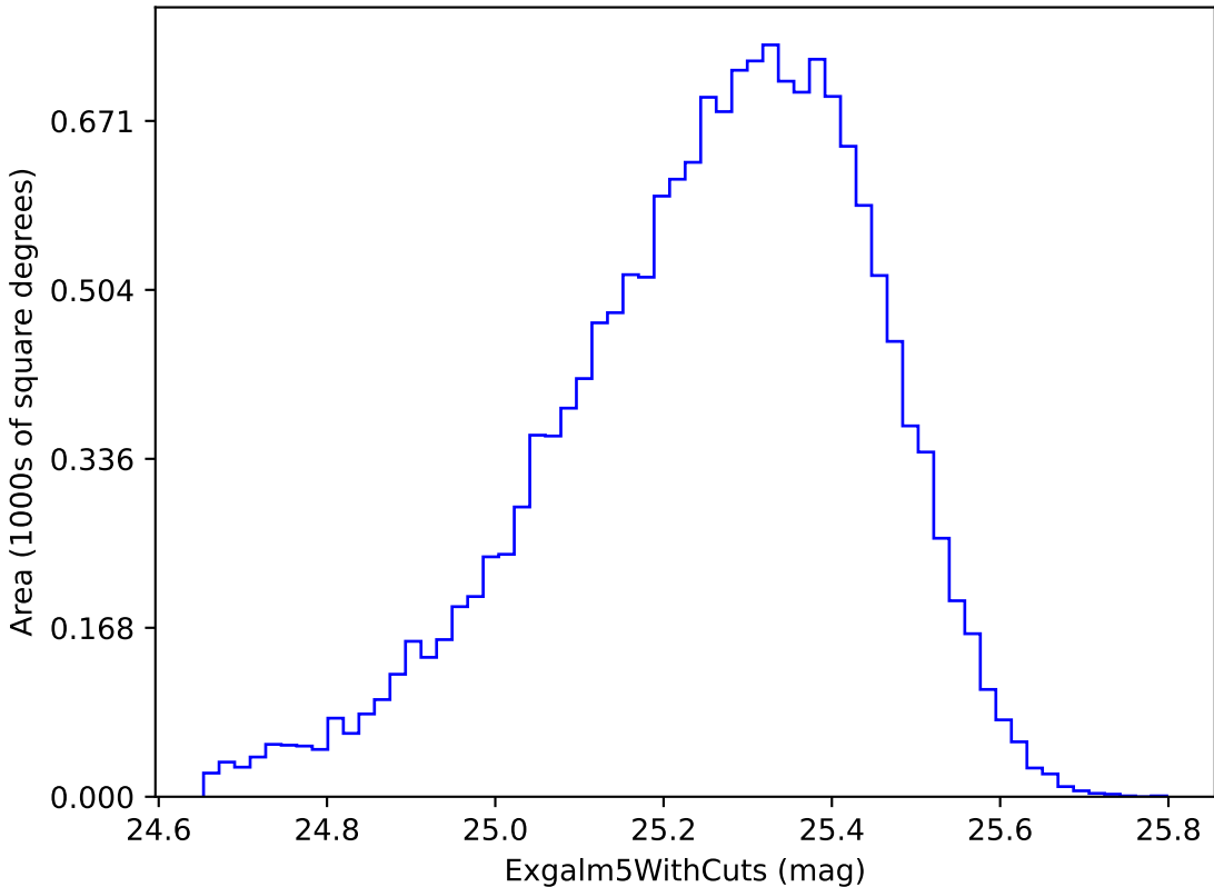
extra_ss_neo3_v3.4_10yrs i band non-DD year 1: ExgalM5WithCuts
