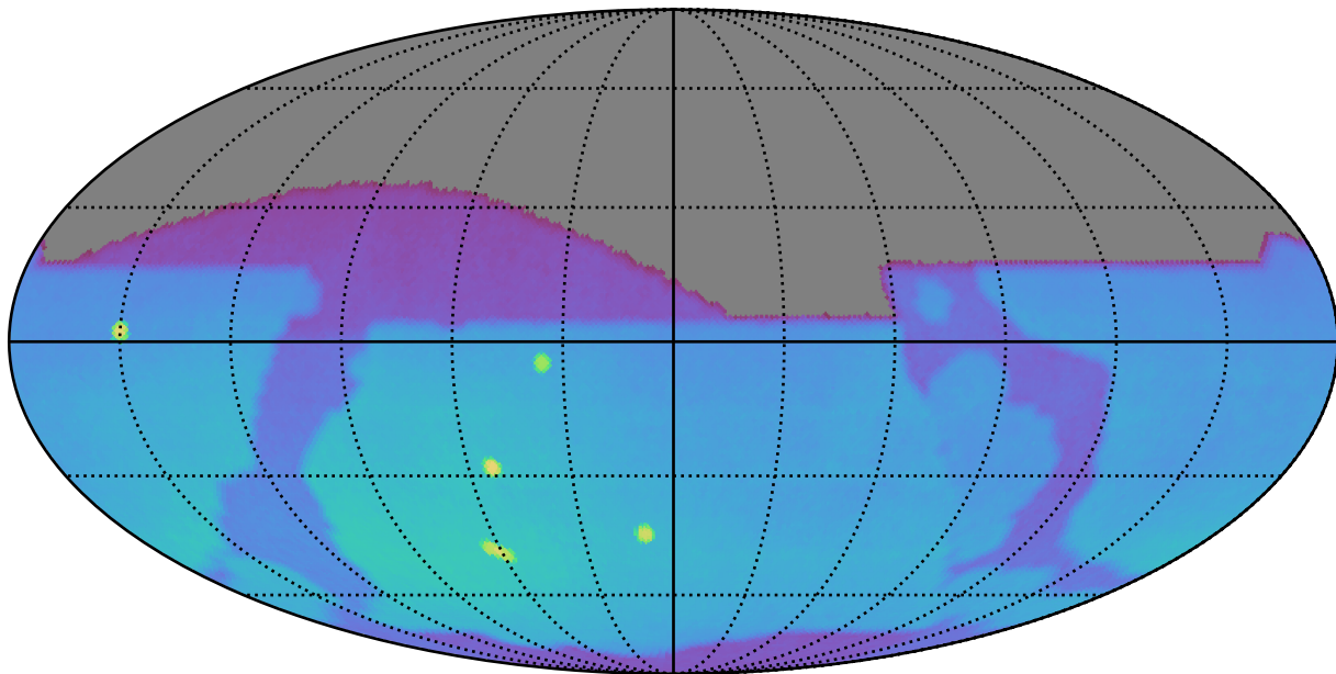
extra_ss_neo3_v3.4_10yrs : Brown Dwarf, L4
