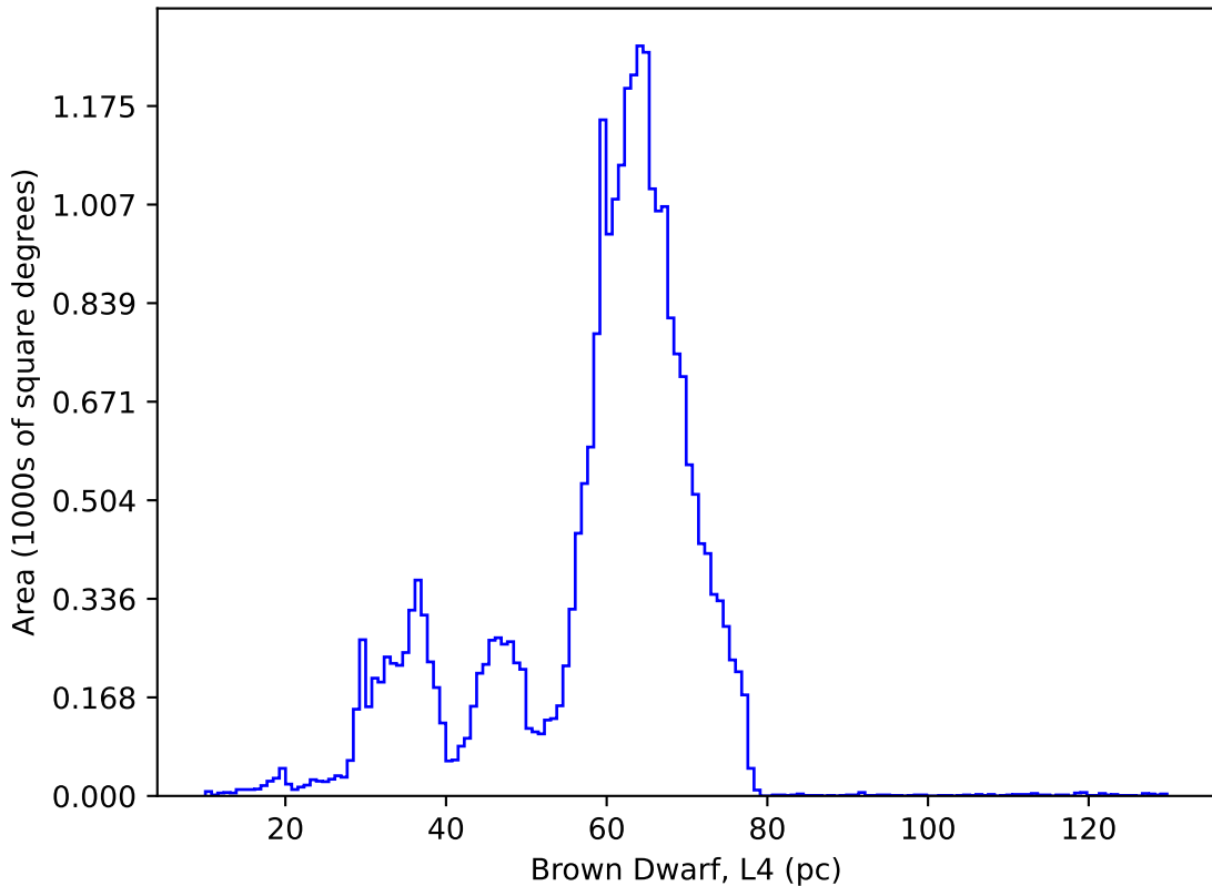
extra_ss_neo3_v3.4_10yrs : Brown Dwarf, L4
