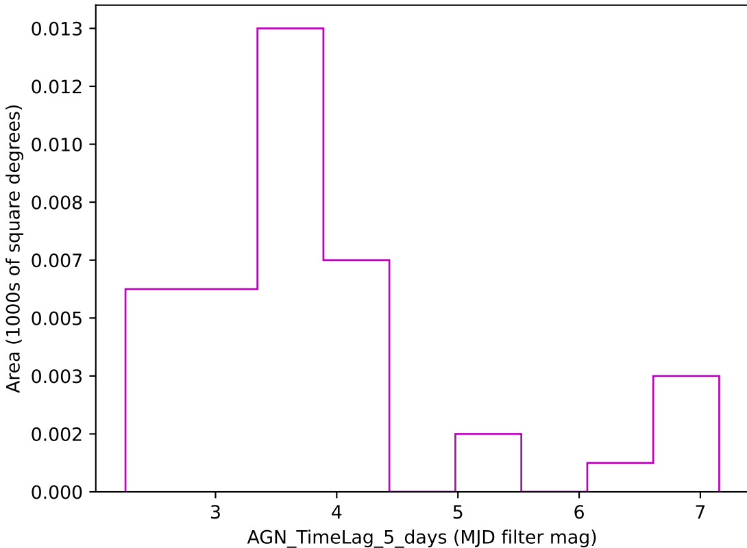
extra_ss_neo3_v3.4_10yrs z band: AGN_TimeLag_5_days
