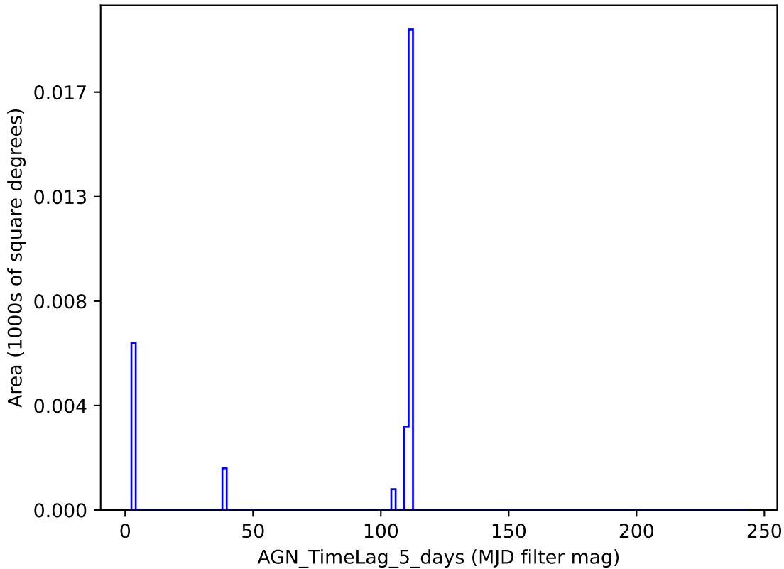
extra_ss_neo3_v3.4_10yrs y band: AGN_TimeLag_5_days
