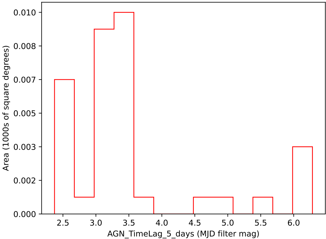
extra_ss_neo3_v3.4_10yrs i band: AGN_TimeLag_5_days
