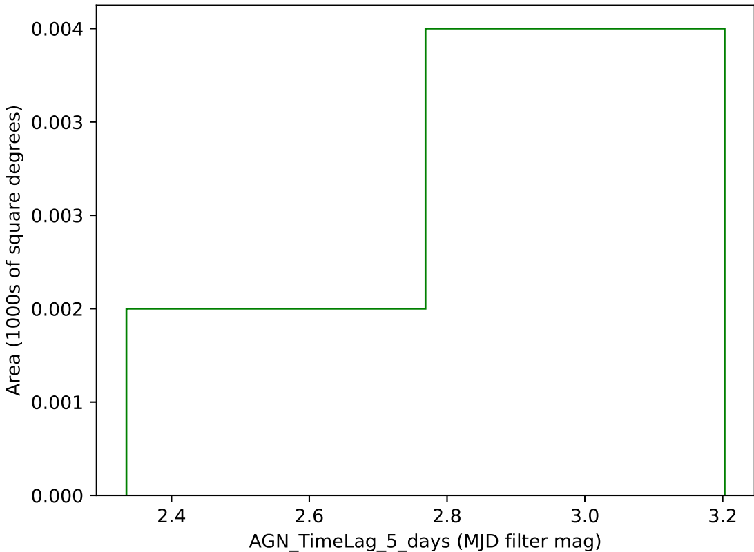
extra_ss_neo3_v3.4_10yrs g band: AGN_TimeLag_5_days
