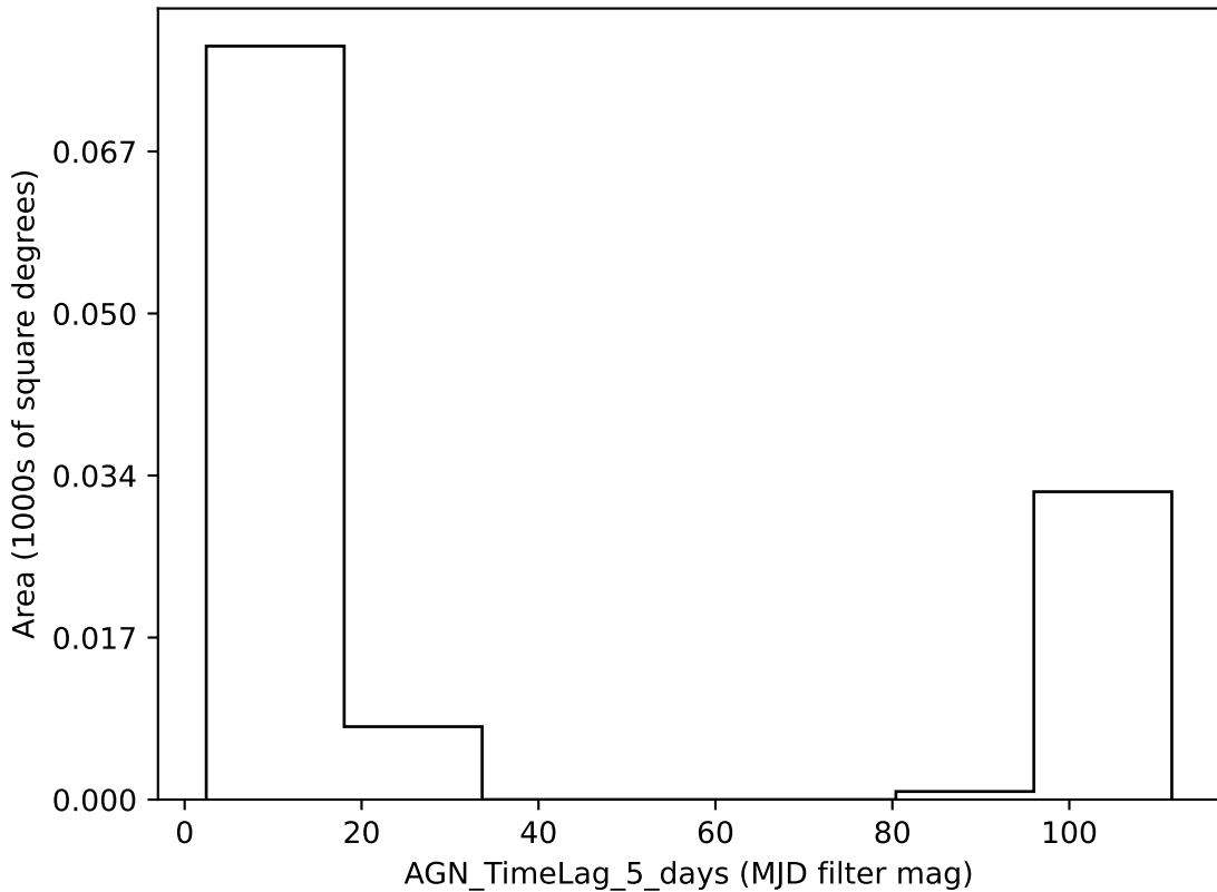
extra_ss_neo3_v3.4_10yrs all bands: AGN_TimeLag_5_days
