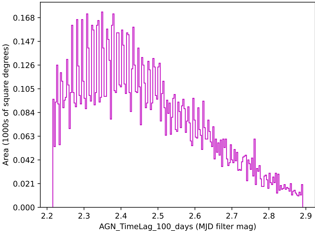
extra_ss_neo3_v3.4_10yrs z band: AGN_TimeLag_100_days
