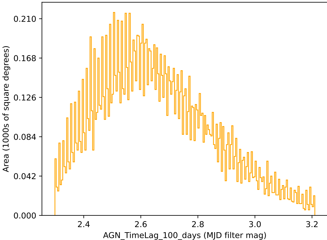
extra_ss_neo3_v3.4_10yrs r band: AGN_TimeLag_100_days
