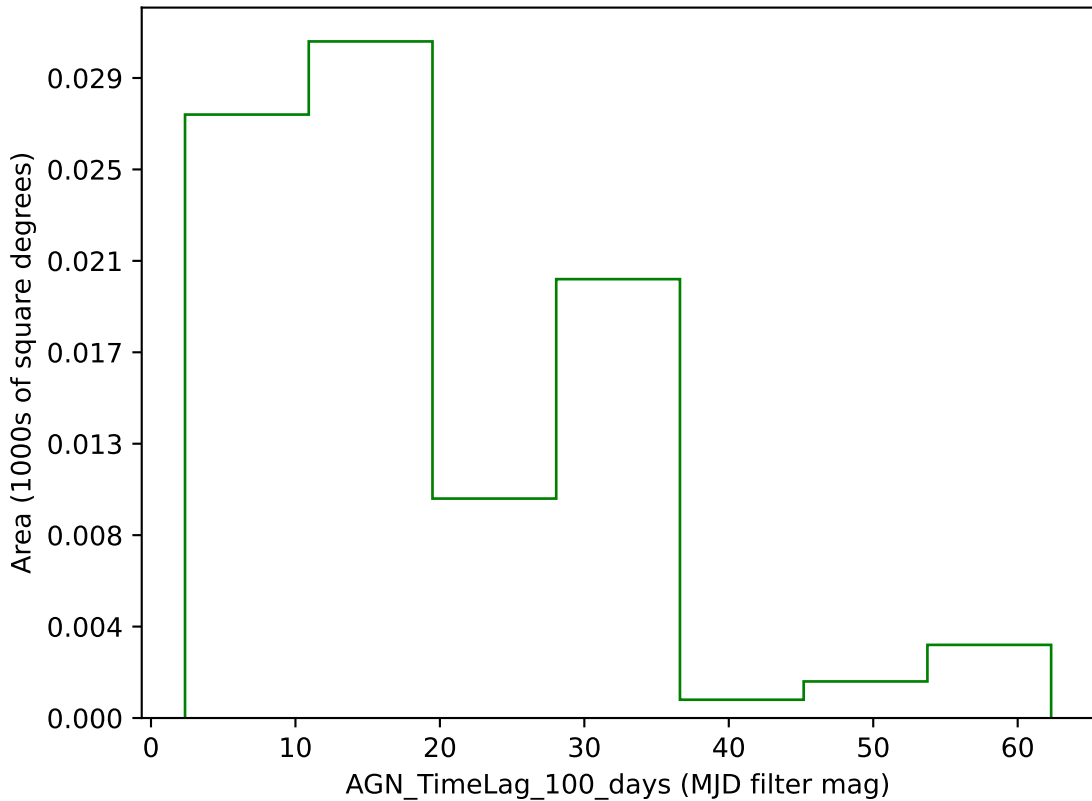
extra_ss_neo3_v3.4_10yrs g band: AGN_TimeLag_100_days
