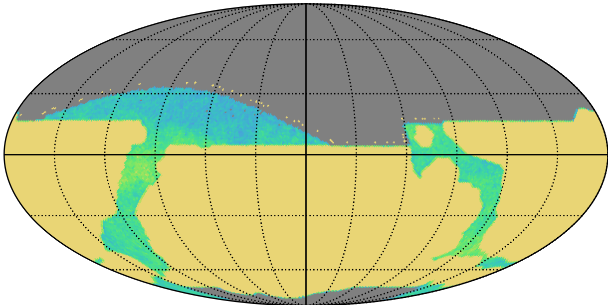
extra_ss_neo3_v3.4_10yrs all bands: AGN_TimeLag_100_days
