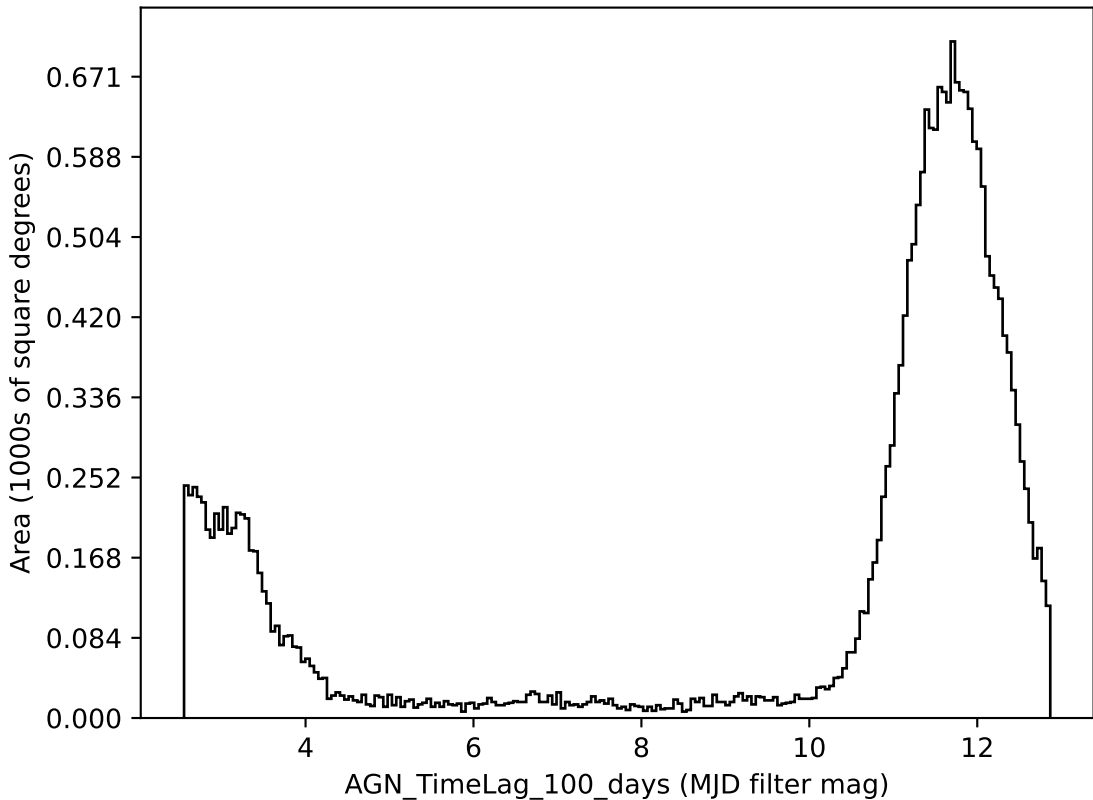
extra_ss_neo3_v3.4_10yrs all bands: AGN_TimeLag_100_days
